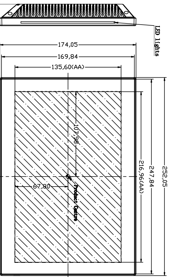
Left view
